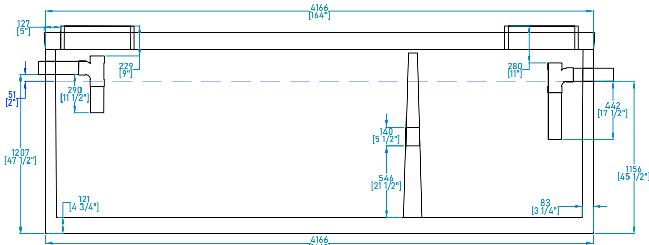
PLAN VIEW - X
