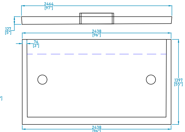
COMPONENT VIEW - Y
