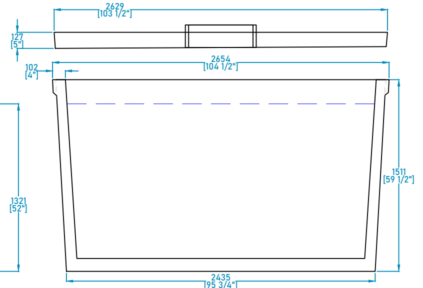
COMPONENT VIEW - Y
